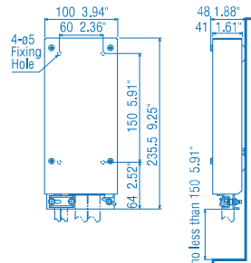
Sensor Adapter (Digital IN) MC-3020D 0.8 kg 1.8 lb
