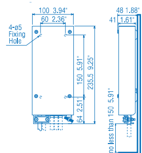
Sensor Adapter (Analog) MC-3010A 0.8 kg 1.8 lb
