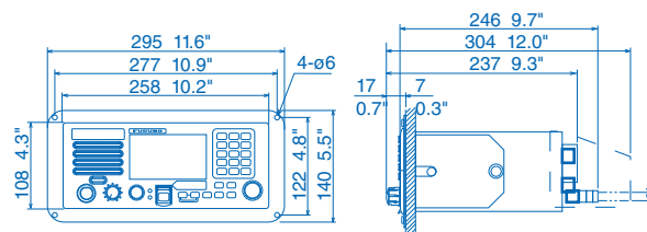
Transceiver Unit (Flush Mount)
