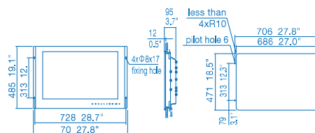
Monitor Unit MU-270W
