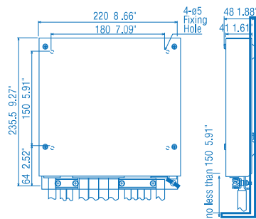
Sensor Adapter (Serial) MC-3000S 1.5 kg 3.3 lb
