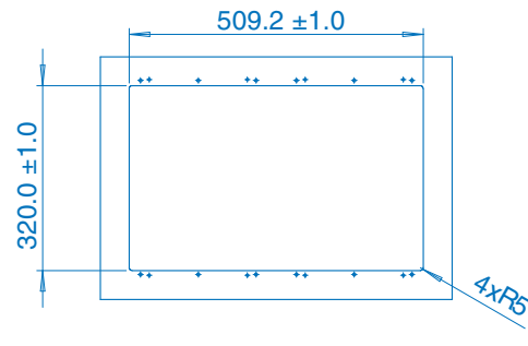
Multi Function Display Flush Mount TZT22X Cutout Dimension
