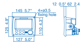
Display Unit FA-1701
