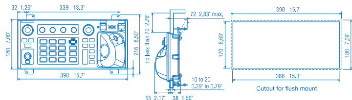
Control Unit RCU-025 3.1kg 6.84 lb
