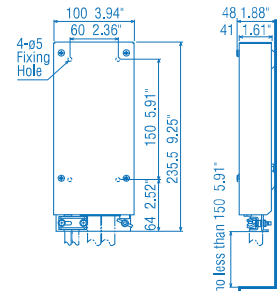
Sensor Adapter (Digital OUT) MC-3030D 0.8 kg 1.8 lb
