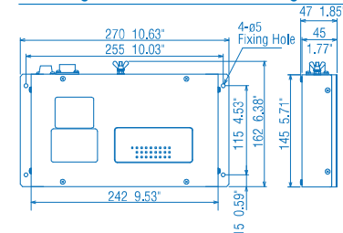
Switching Hub HUB-100 1.5 kg 3.31 lb
