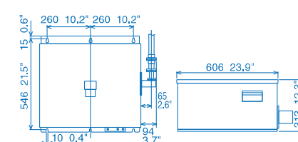
Transceiver Unit RTR-109 22 kg 48.5 lb
