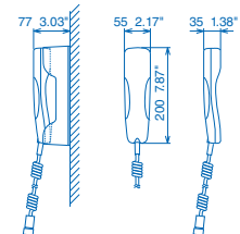
Headset HS-2003 0.5 kg 1.2 lb
