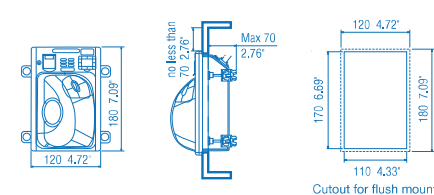
Trackball Control Unit RCU-026 1.5 kg 3.31 lb
