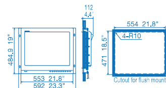
Monitor Unit MU-231 12.8 kg 28.2 lb
