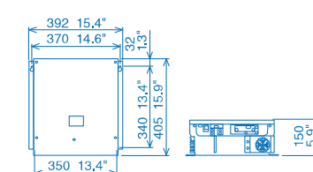
Power Supply Unit PSU-015/018 10 kg 22 lb
