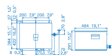
Power Supply Unit PSU-014/016 8.5 kg 18.7 lb
