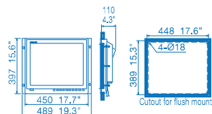
Monitor Unit MU-190 8.8 kg 19.4 lb
